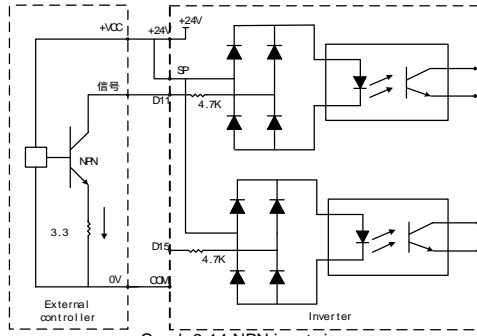
Graph 2-14 NPN input wiring
