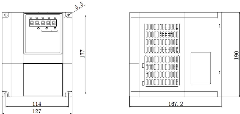
Graph 1-4 2.2KW ~ 3.7KW product outline & dimensions
