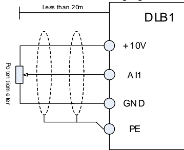
Graph 2-12 Analog input terminal wiring
