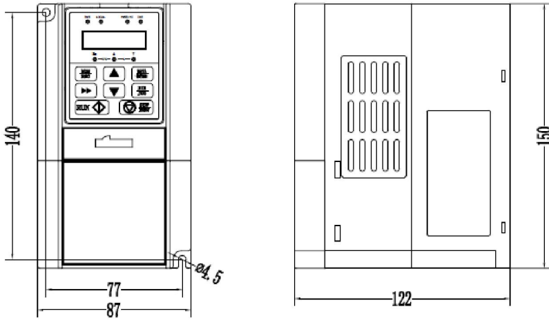
Graph 1-3 0.4W~1.5KW product outlines & dimensions
