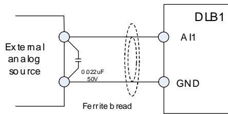
Graph 2-13 Analog input terminal treatment
