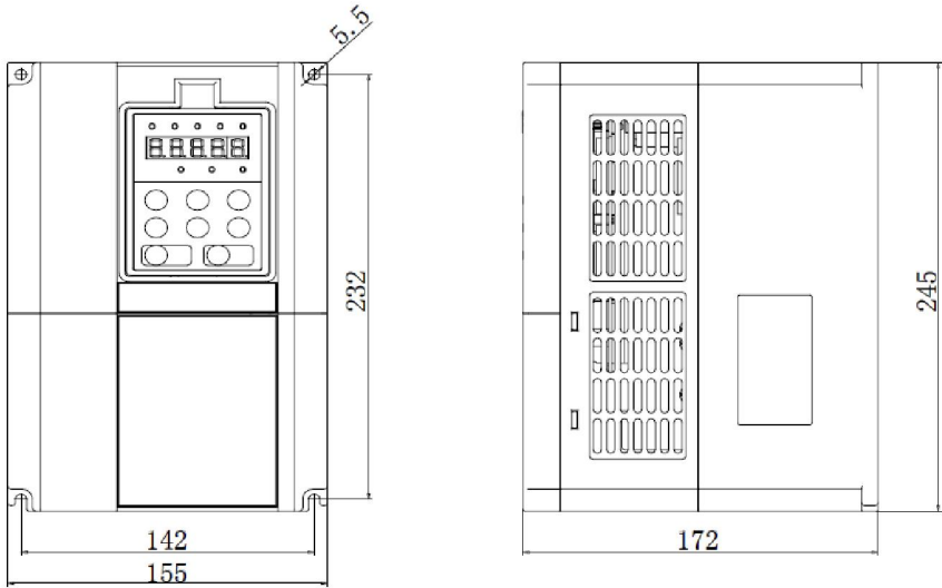
Graph 1-5 5.5 ~ 7.5KW product outline & dimensions
