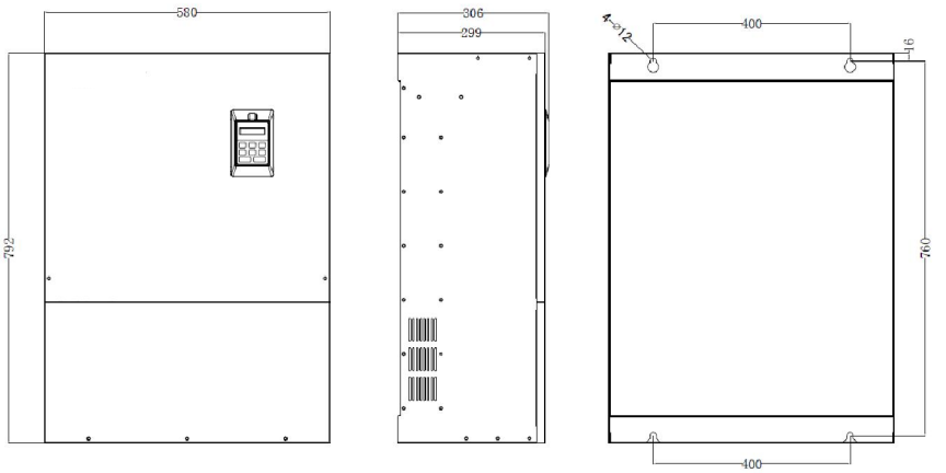
Graph 1-9 132 ~ 160KW product outline & dimensions
