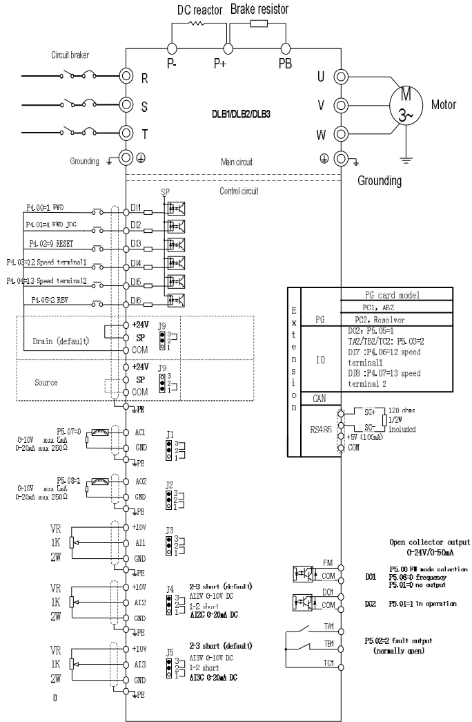
Graph 2-922 ~ 400KW inverter wiring diagram
